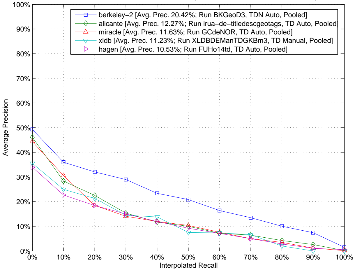
CLEF 2005 – Top 5 participants of GeoCLEF Monolingual DE – Interpolated Recall vs Average Precision
