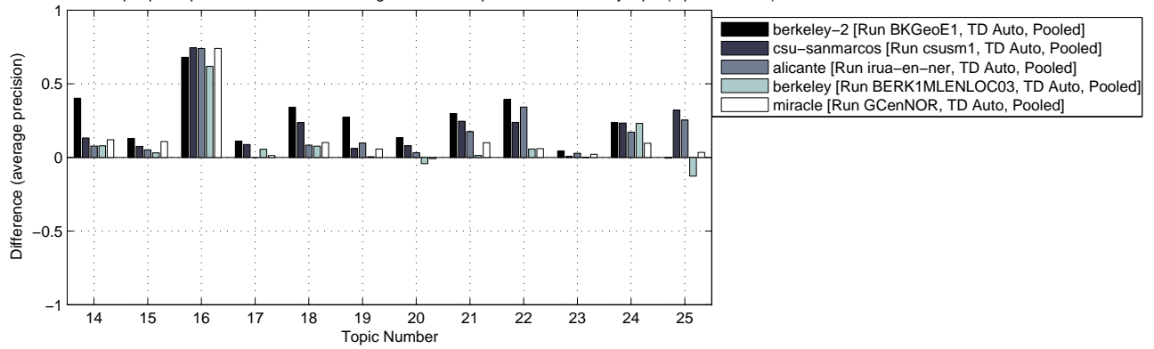
CLEF 2005 – Top 5 participants of GeoCLEF Monolingual EN – Comparison to median by topic (topics 14 to 25)
