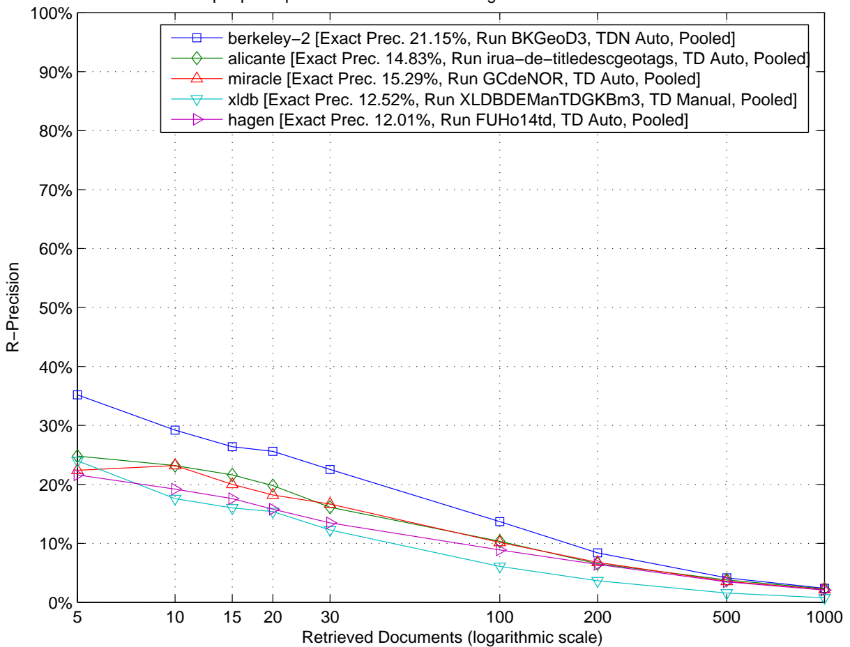
CLEF 2005 – Top 5 participants of GeoCLEF Monolingual DE – Retrieved documents vs Precision
