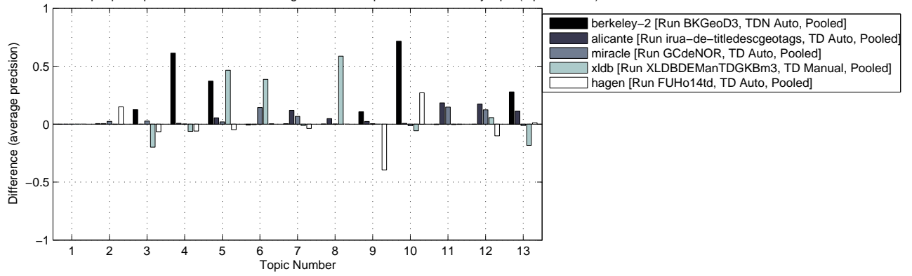
CLEF 2005 – Top 5 participants of GeoCLEF Monolingual DE – Comparison to median by topic (topics 1 to 13)
