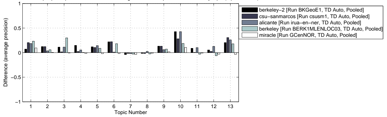
CLEF 2005 – Top 5 participants of GeoCLEF Monolingual EN – Comparison to median by topic (topics 1 to 13)
