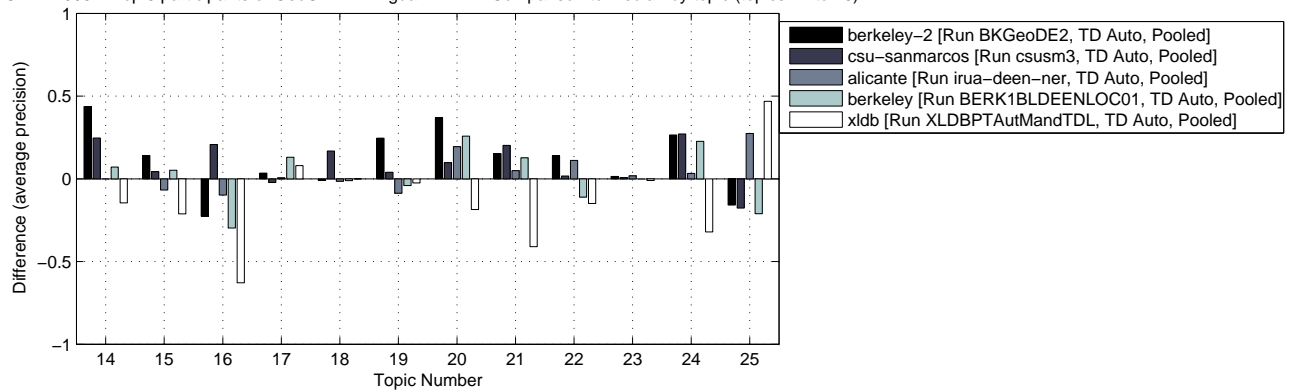
CLEF 2005 – Top 5 participants of GeoCLEF Bilingual X2EN – Comparison to median by topic (topics 14 to 25)
