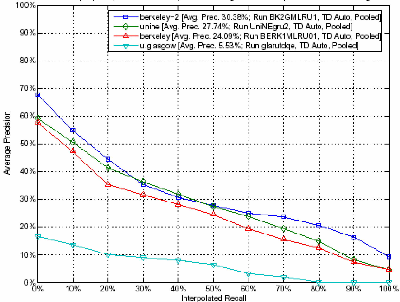
CLEF 2005 – Top 4 participants of Domain Specific Monolingual RU – Interpolated Recall vs Average Precision
